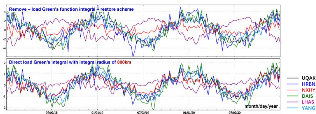
Fig 3.11 Surface atmosphere load effect time series on ground gravity (mGal) at 6 CORS stations in mainland China using two scheme
