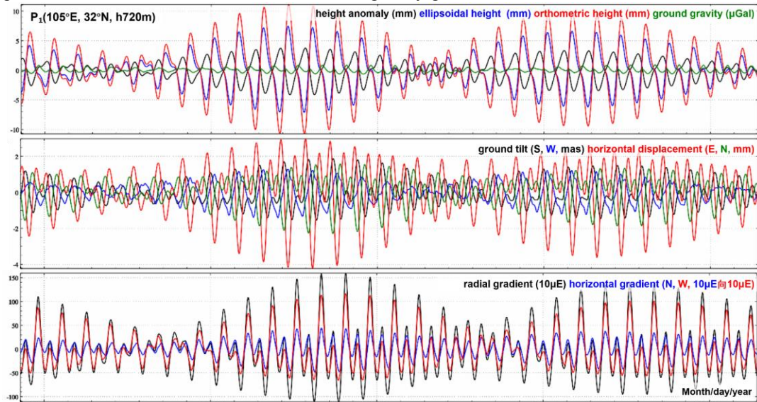
Fig 4.3 The ocean tidal load effect time series on geodetic variations at P_1 point in the inland area
