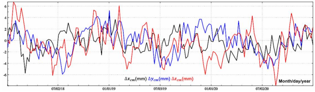
Fig 5.6 The surface atmosphere variation load effect time series on Earth's mass centric variation (relative to the mean center of mass in 2018)
